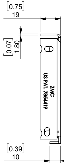
RS-UJA,B,C,D,E 4" Adj. Fascia Bracket for 1 1/2" RS Clutch
